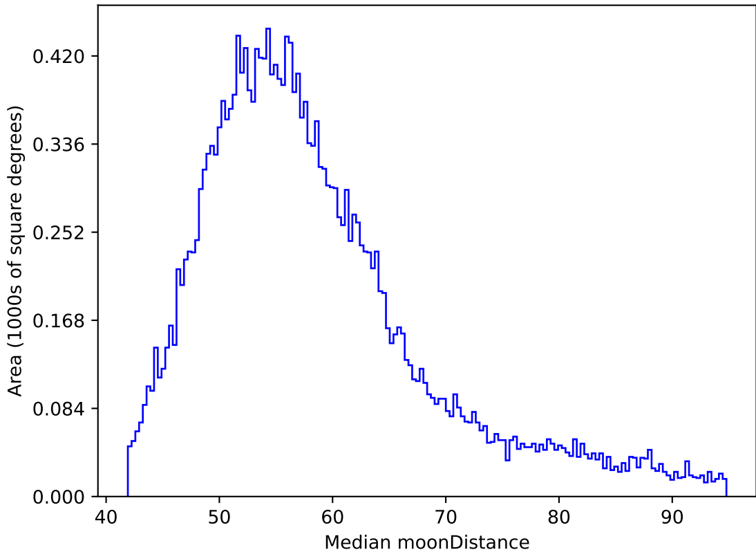
roll_pause_mjdp180_v3.4_10yrs All sky y band: Median moonDistance
