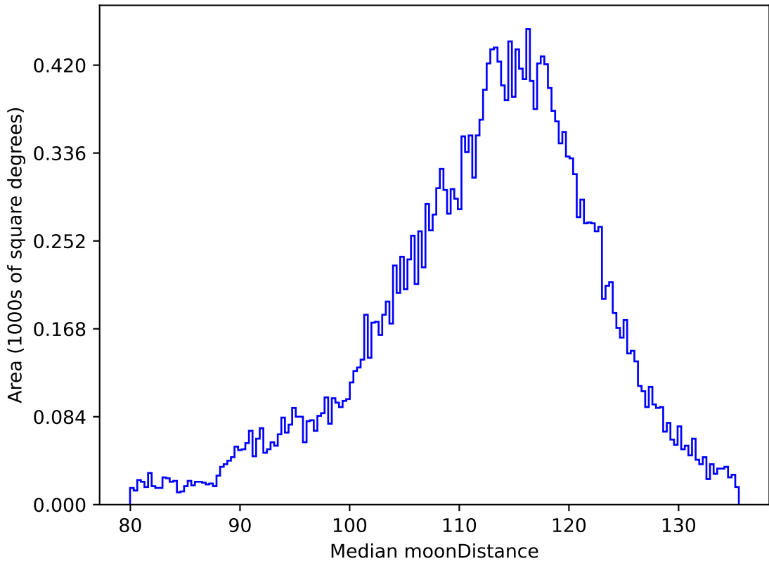
roll_pause_mjdp180_v3.4_10yrs All sky r band: Median moonDistance
