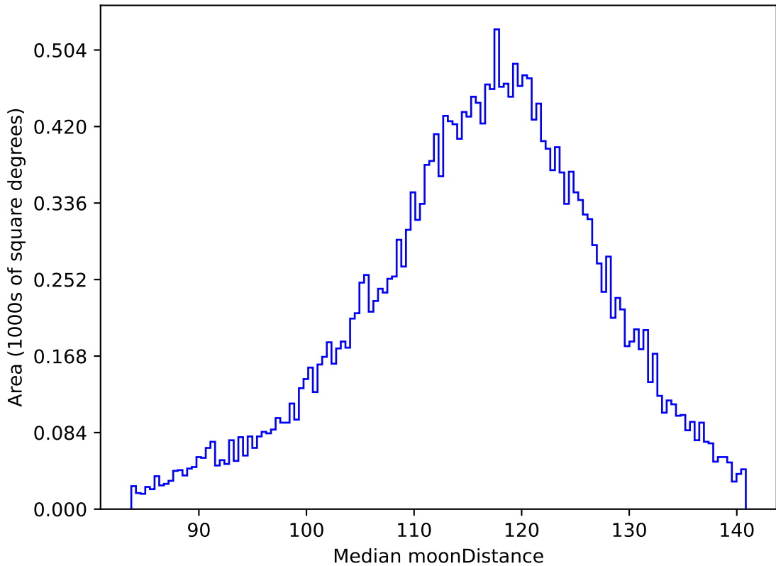
roll_pause_mjdp180_v3.4_10yrs All sky g band: Median moonDistance
