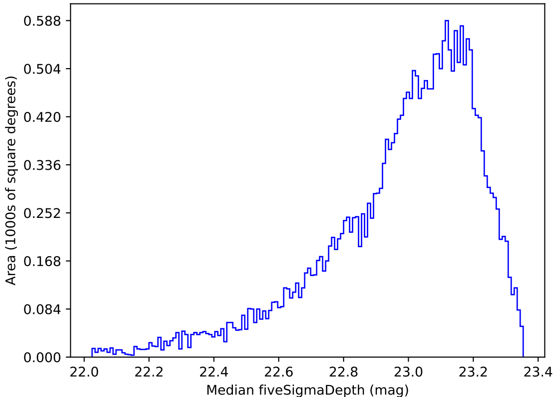
roll_pause_mjdp180_v3.4_10yrs Yr 1 z band: Median fiveSigmaDepth
