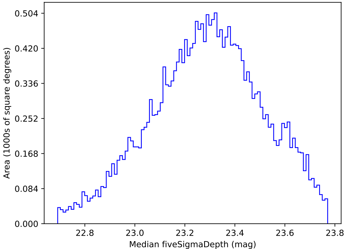
roll_pause_mjdp180_v3.4_10yrs Yr 1 u band: Median fiveSigmaDepth
