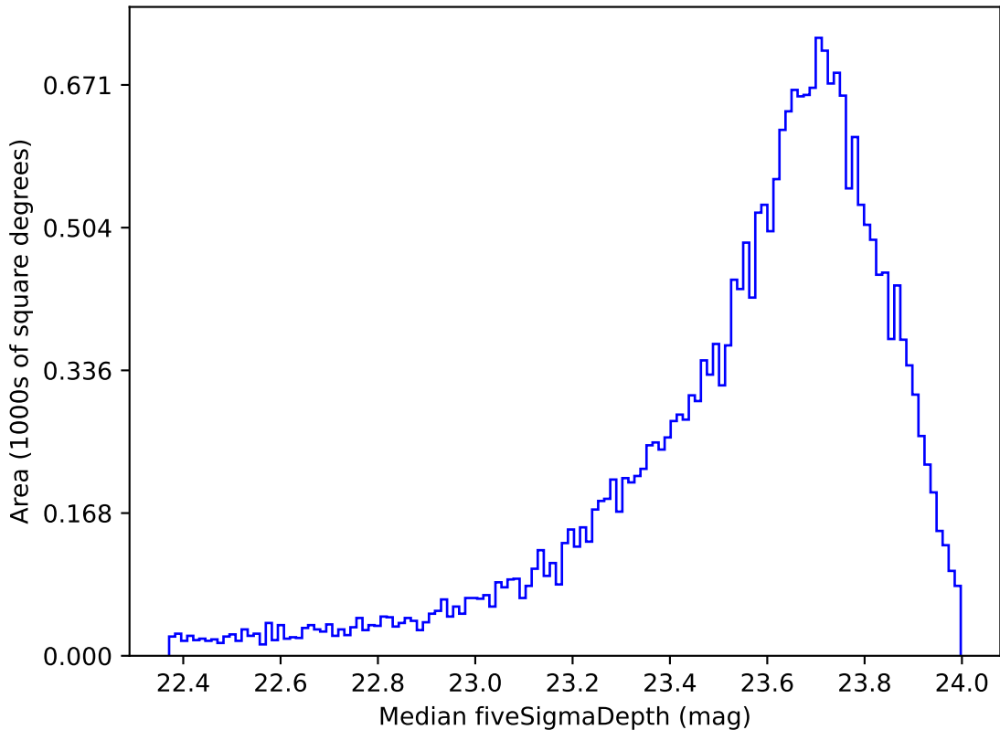
roll_pause_mjdp180_v3.4_10yrs Yr 1 i band: Median fiveSigmaDepth
