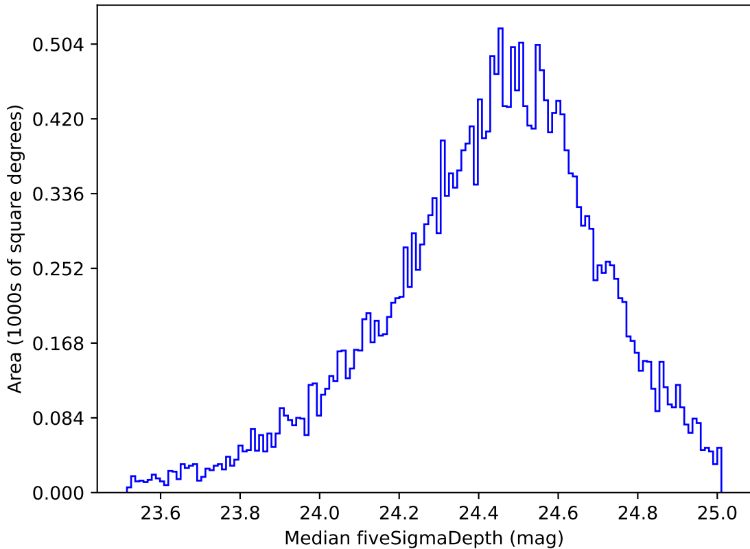
roll_pause_mjdp180_v3.4_10yrs Yr 1 g band: Median fiveSigmaDepth
