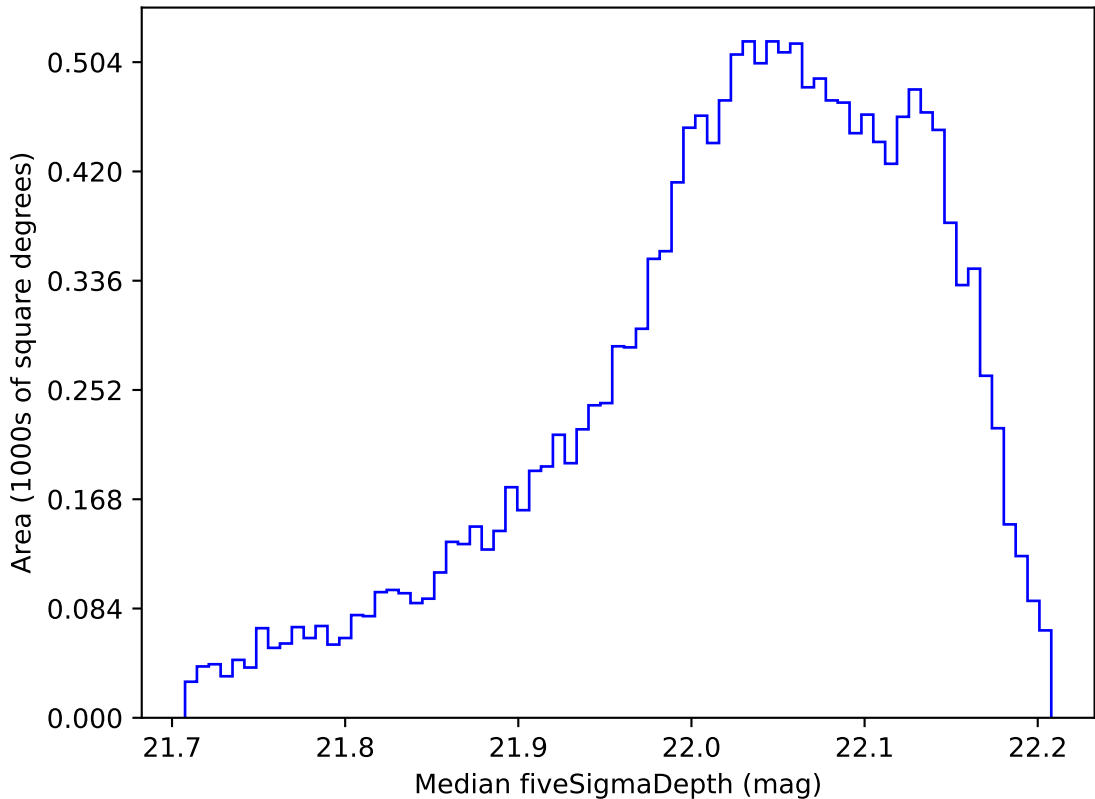
roll_pause_mjdp180_v3.4_10yrs WFD y band: Median fiveSigmaDepth
