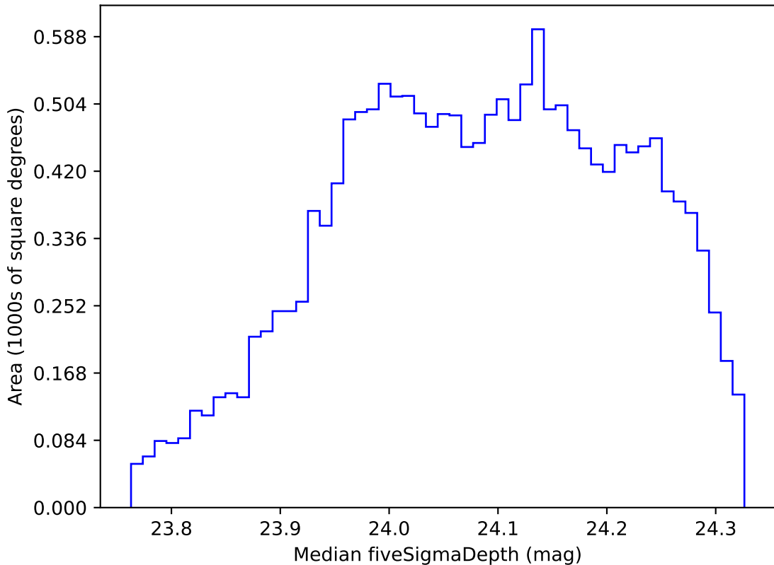
roll_pause_mjdp180_v3.4_10yrs WFD r band: Median fiveSigmaDepth
