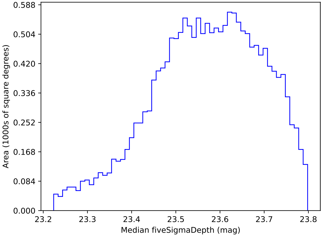
roll_pause_mjdp180_v3.4_10yrs WFD i band: Median fiveSigmaDepth
