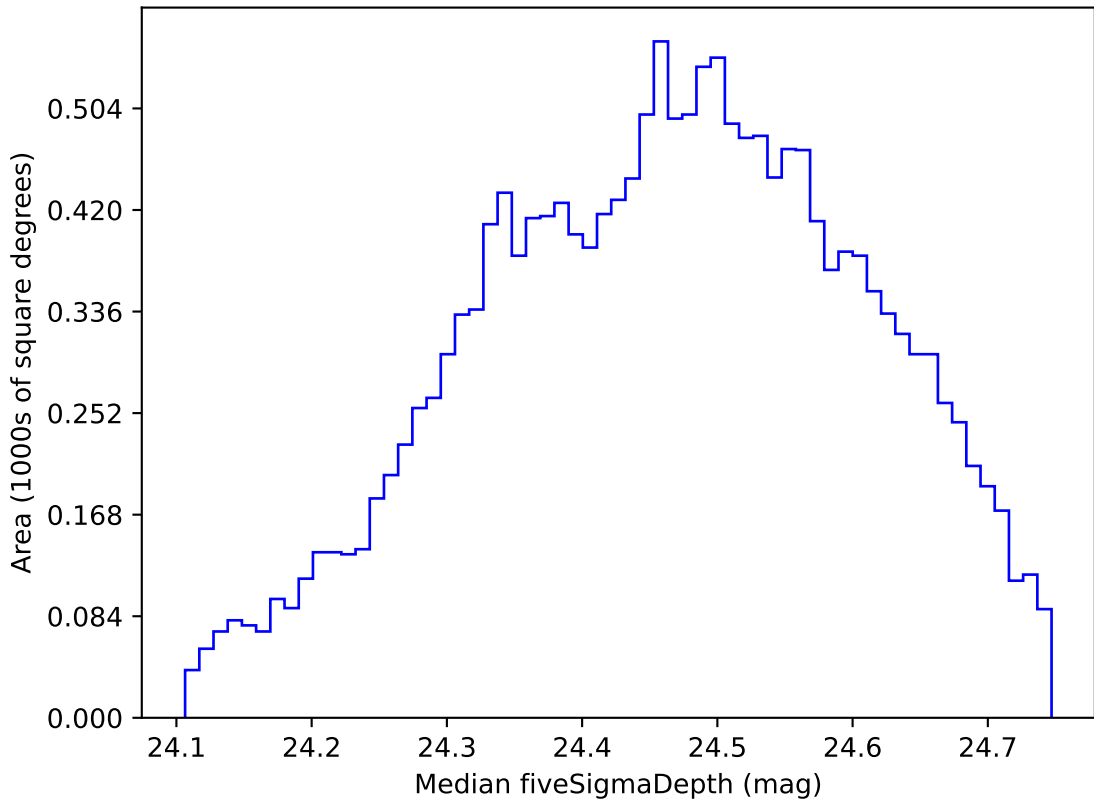
roll_pause_mjdp180_v3.4_10yrs WFD g band: Median fiveSigmaDepth
