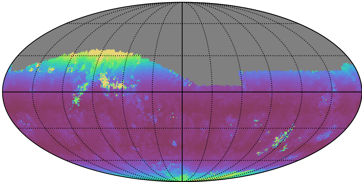
roll_pause_mjdp180_v3.4_10yrs Yr 1 z band: Median airmass
