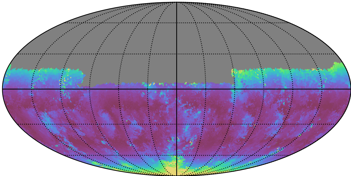
roll_pause_mjdp180_v3.4_10yrs Yr 1 u band: Median airmass
