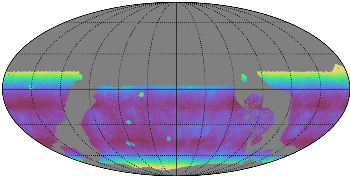
roll_pause_mjdp180_v3.4_10yrs WFD z band: Median airmass
