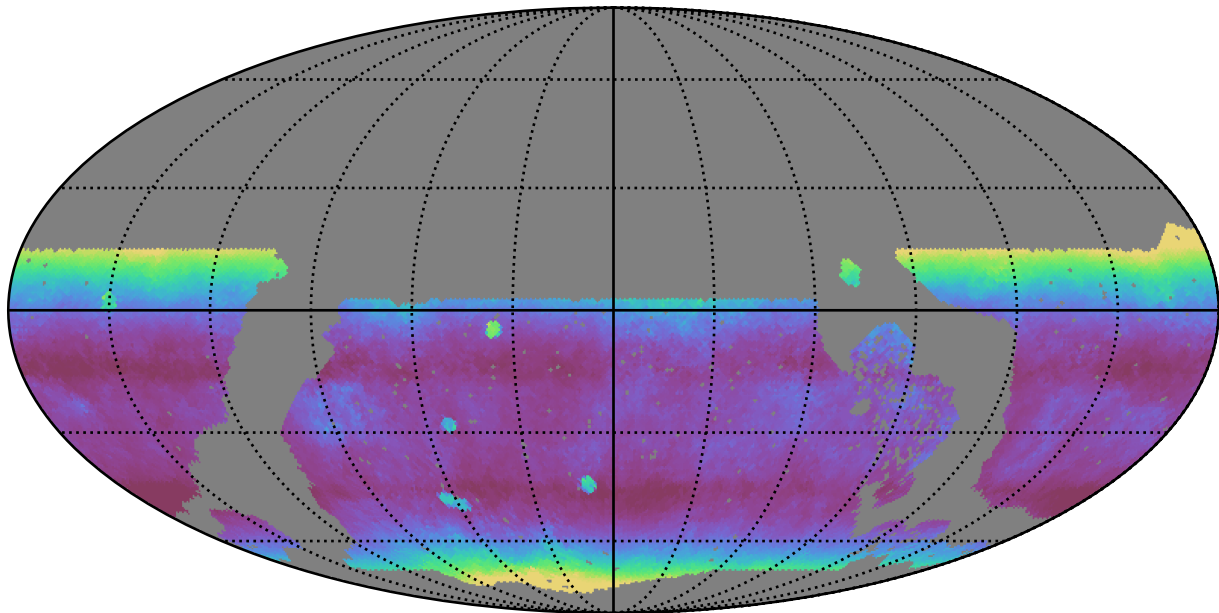
roll_pause_mjdp180_v3.4_10yrs WFD y band: Median airmass
