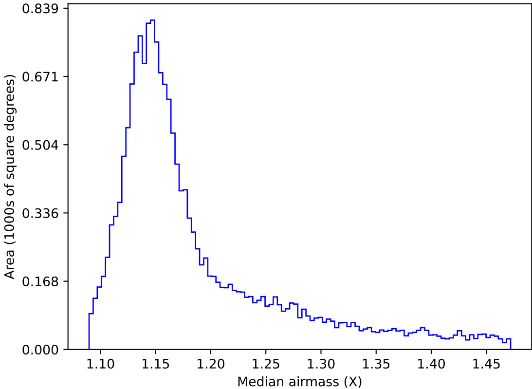
roll_pause_mjdp180_v3.4_10yrs WFD y band: Median airmass
