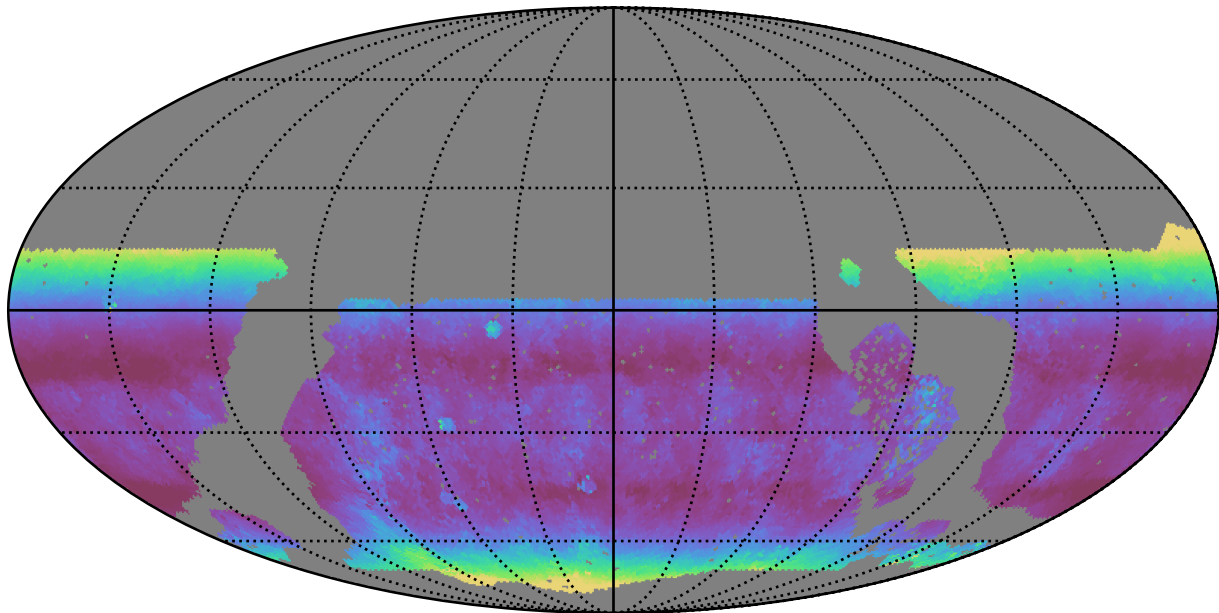
roll_pause_mjdp180_v3.4_10yrs WFD u band: Median airmass
