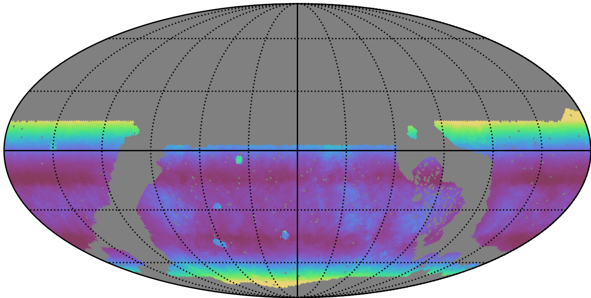
roll_pause_mjdp180_v3.4_10yrs WFD r band: Median airmass
