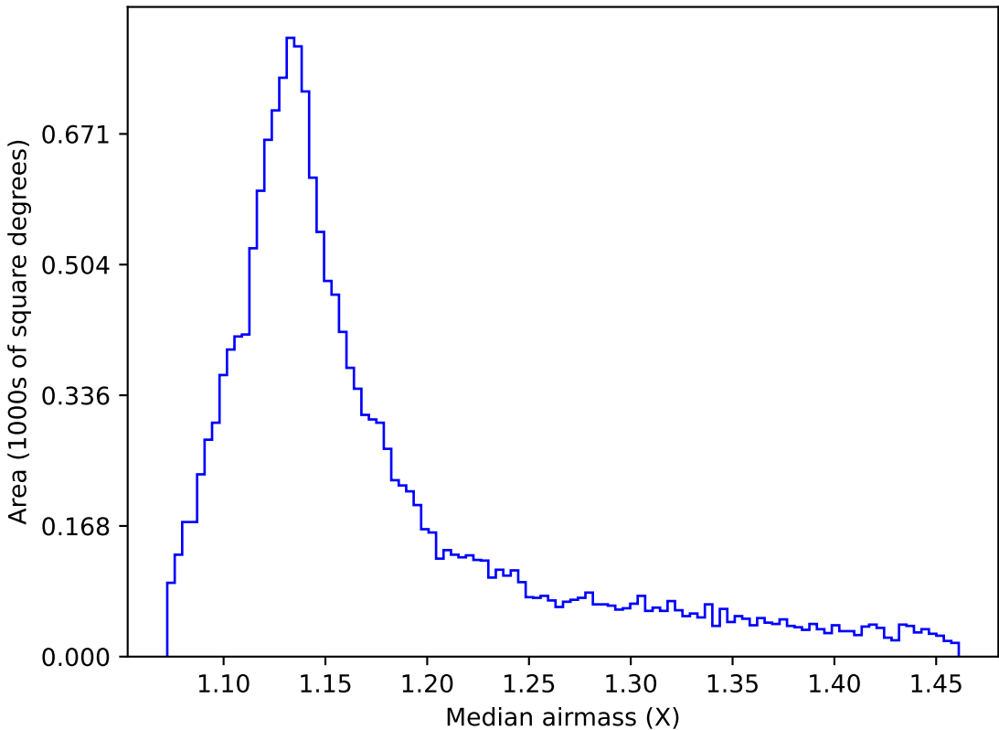
roll_pause_mjdp180_v3.4_10yrs WFD r band: Median airmass
