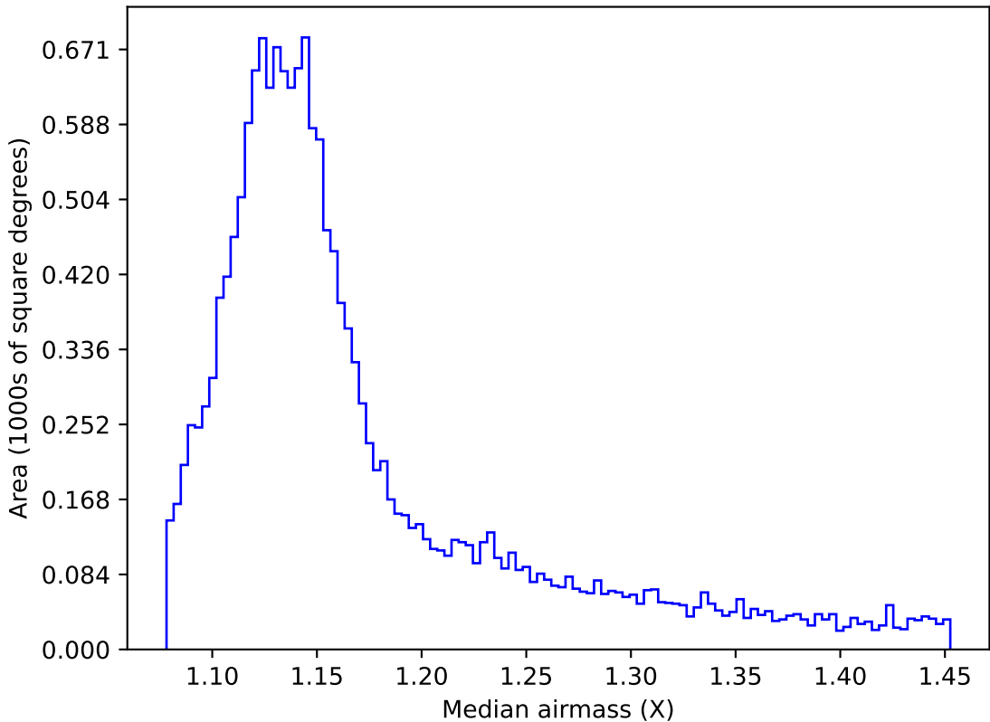
roll_pause_mjdp180_v3.4_10yrs WFD i band: Median airmass
