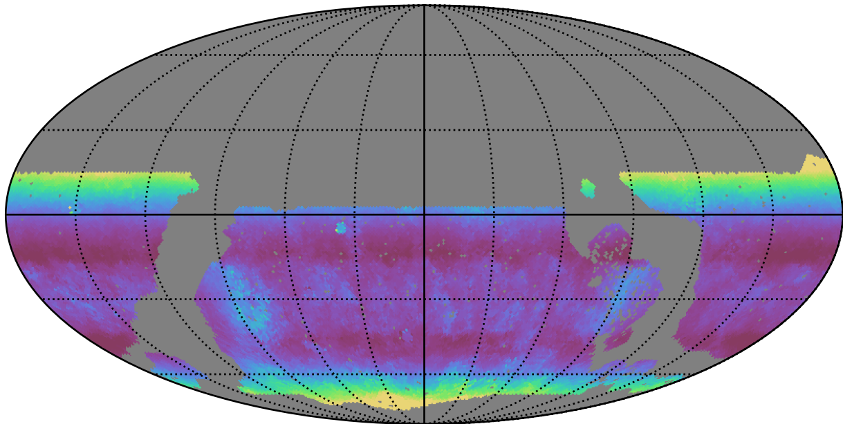
roll_pause_mjdp180_v3.4_10yrs WFD g band: Median airmass
