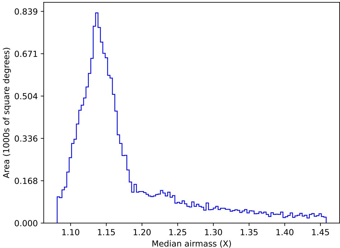
roll_pause_mjdp180_v3.4_10yrs WFD all bands: Median airmass
