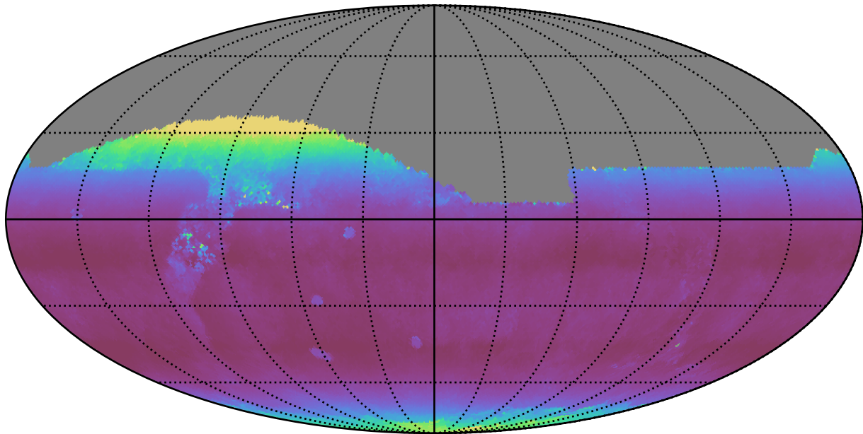
roll_pause_mjdp180_v3.4_10yrs All sky z band: Median airmass
