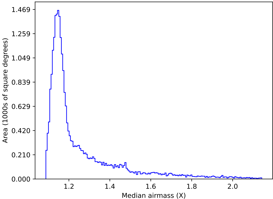
roll_pause_mjdp180_v3.4_10yrs All sky z band: Median airmass
