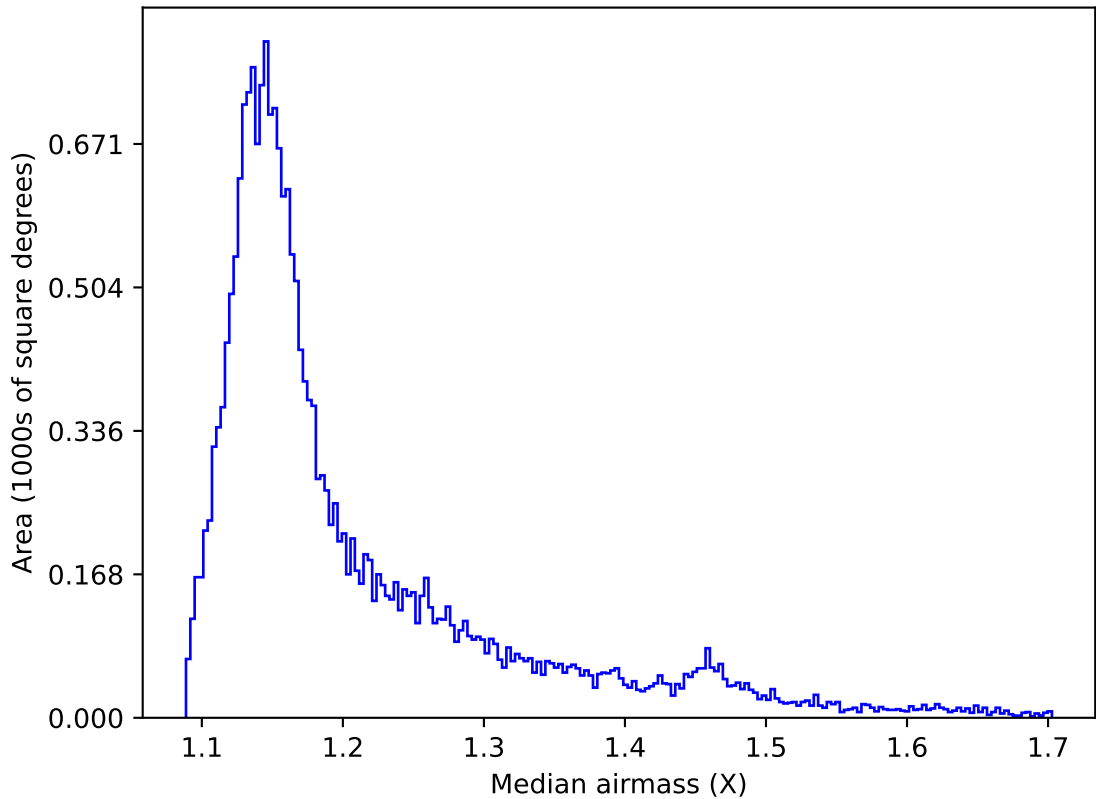
roll_pause_mjdp180_v3.4_10yrs All sky y band: Median airmass
