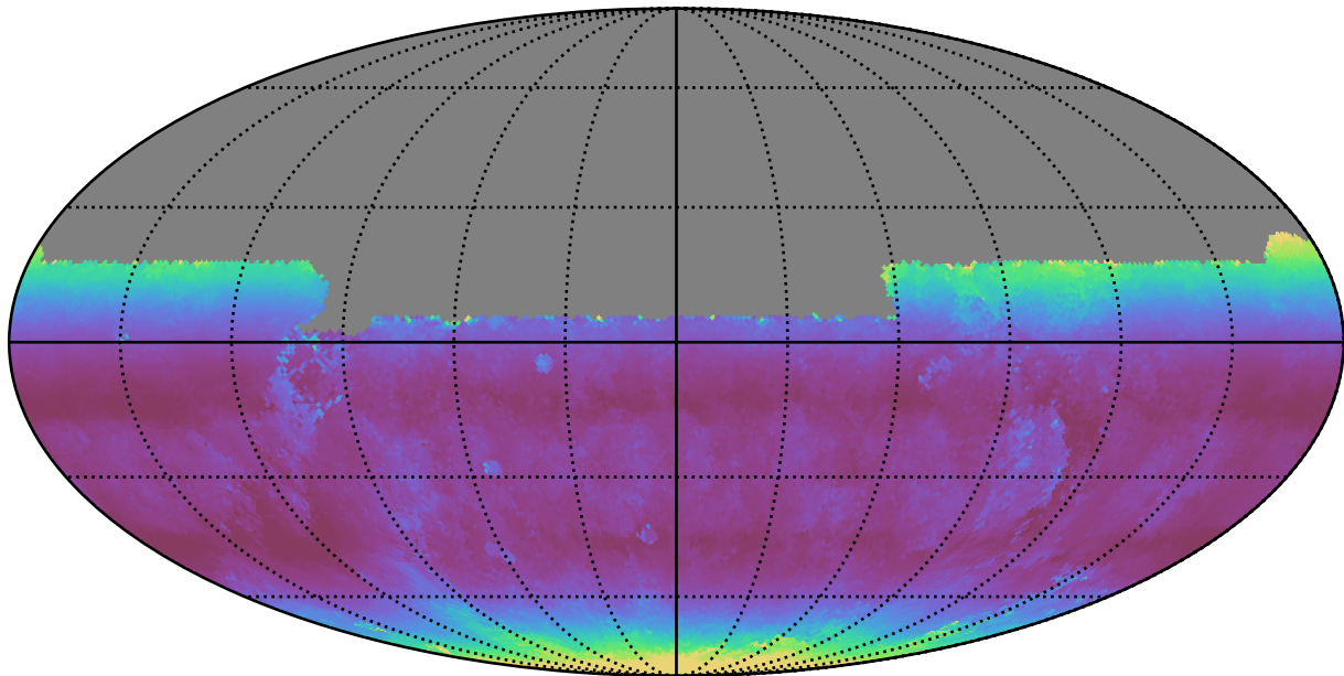
roll_pause_mjdp180_v3.4_10yrs All sky u band: Median airmass
