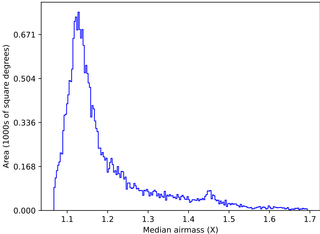
roll_pause_mjdp180_v3.4_10yrs All sky u band: Median airmass
