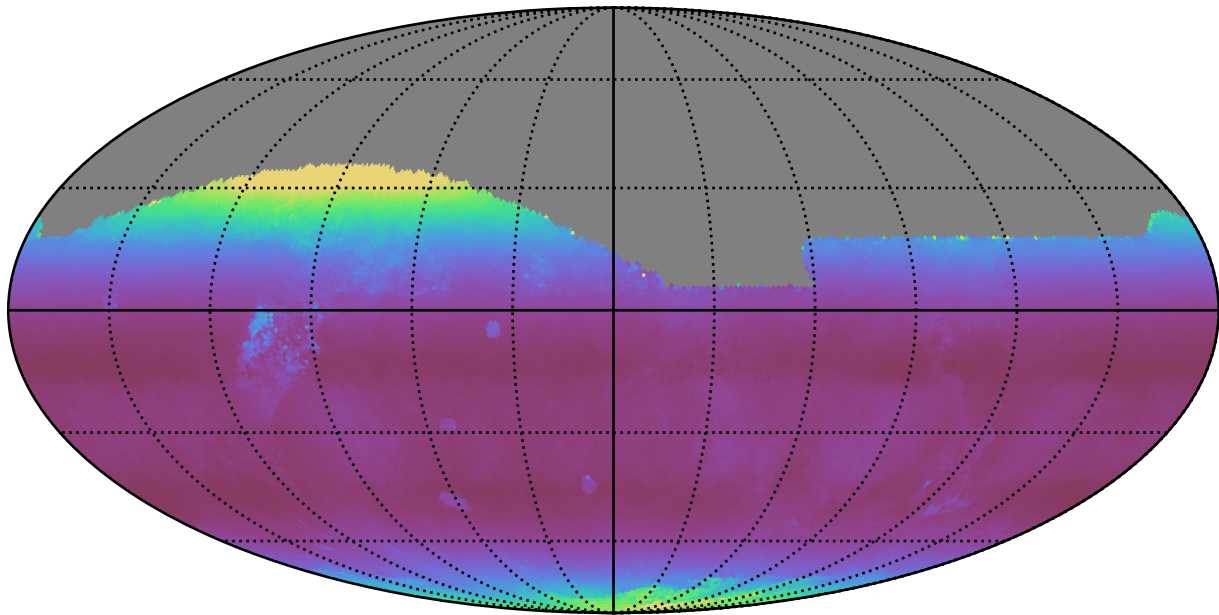
roll_pause_mjdp180_v3.4_10yrs All sky r band: Median airmass
