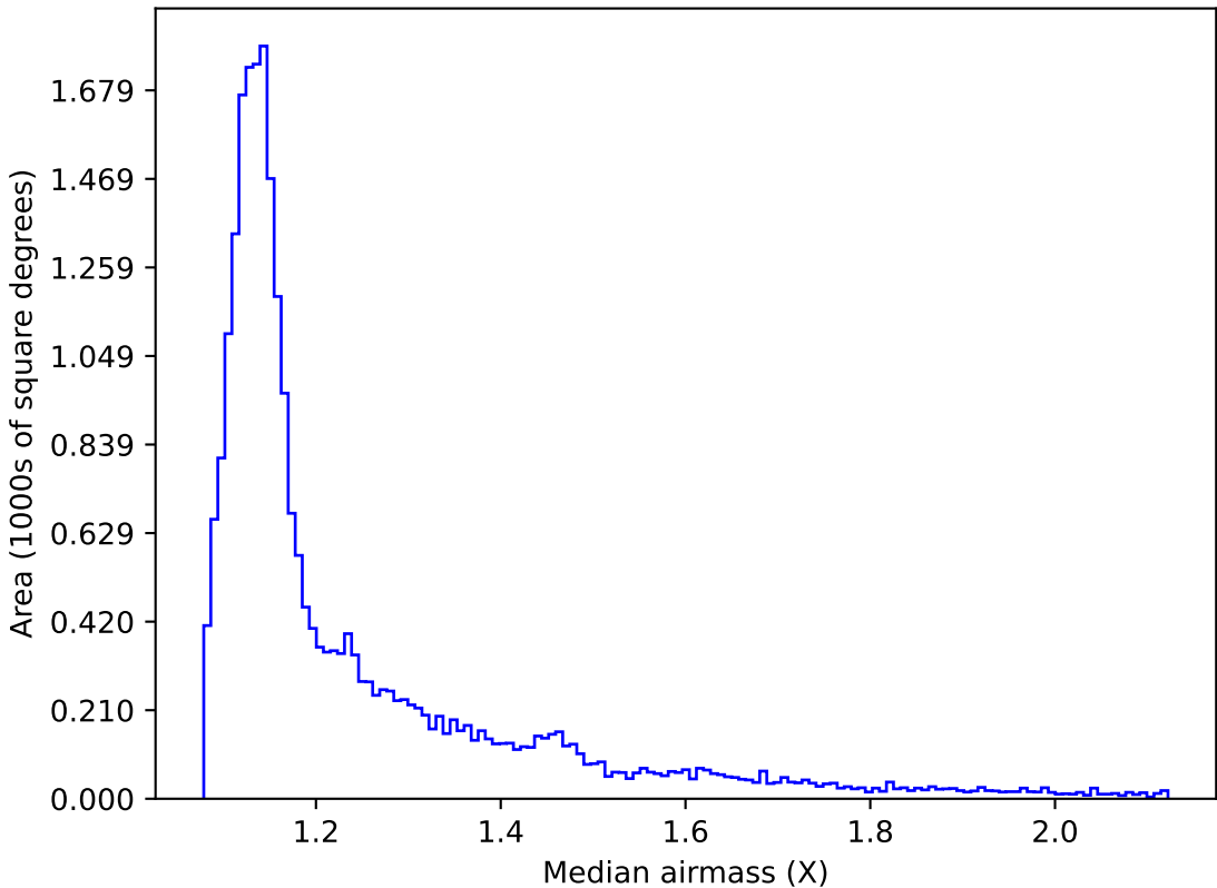
roll_pause_mjdp180_v3.4_10yrs All sky i band: Median airmass
