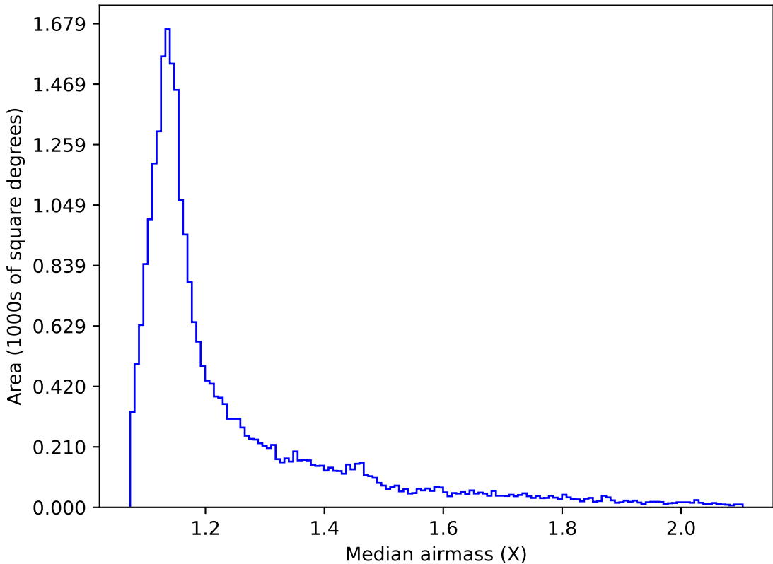
roll_pause_mjdp180_v3.4_10yrs All sky g band: Median airmass
