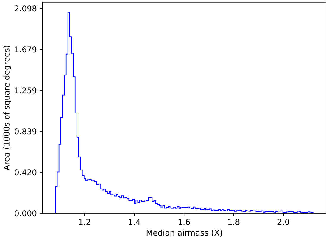
roll_pause_mjdp180_v3.4_10yrs All sky all bands: Median airmass
