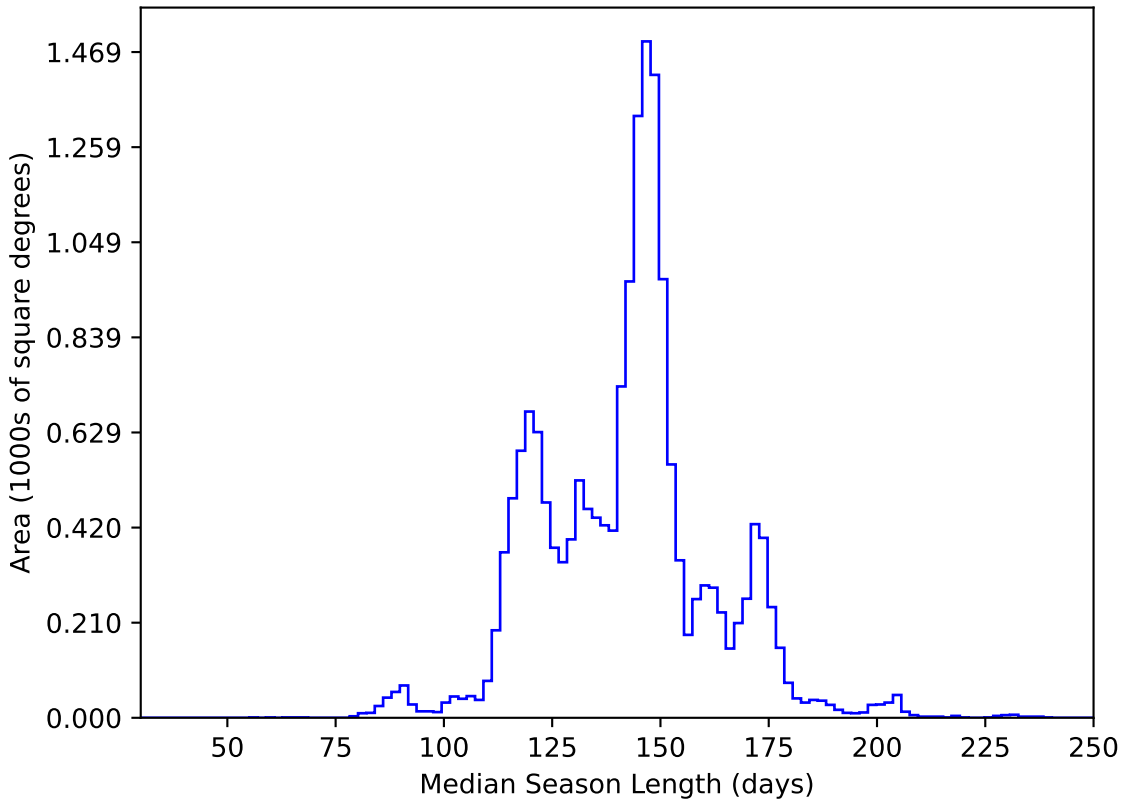
roll_pause_mjdp180_v3.4_10yrs WFD y band: Median Season Length
