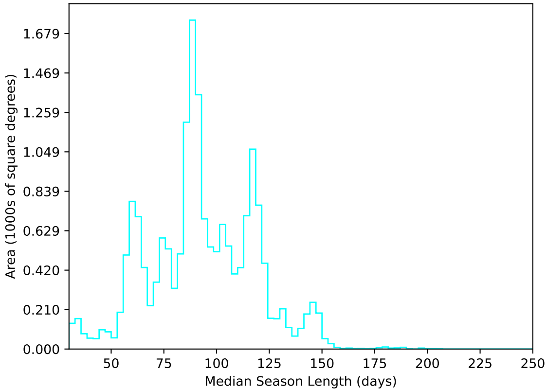
roll_pause_mjdp180_v3.4_10yrs WFD u band: Median Season Length
