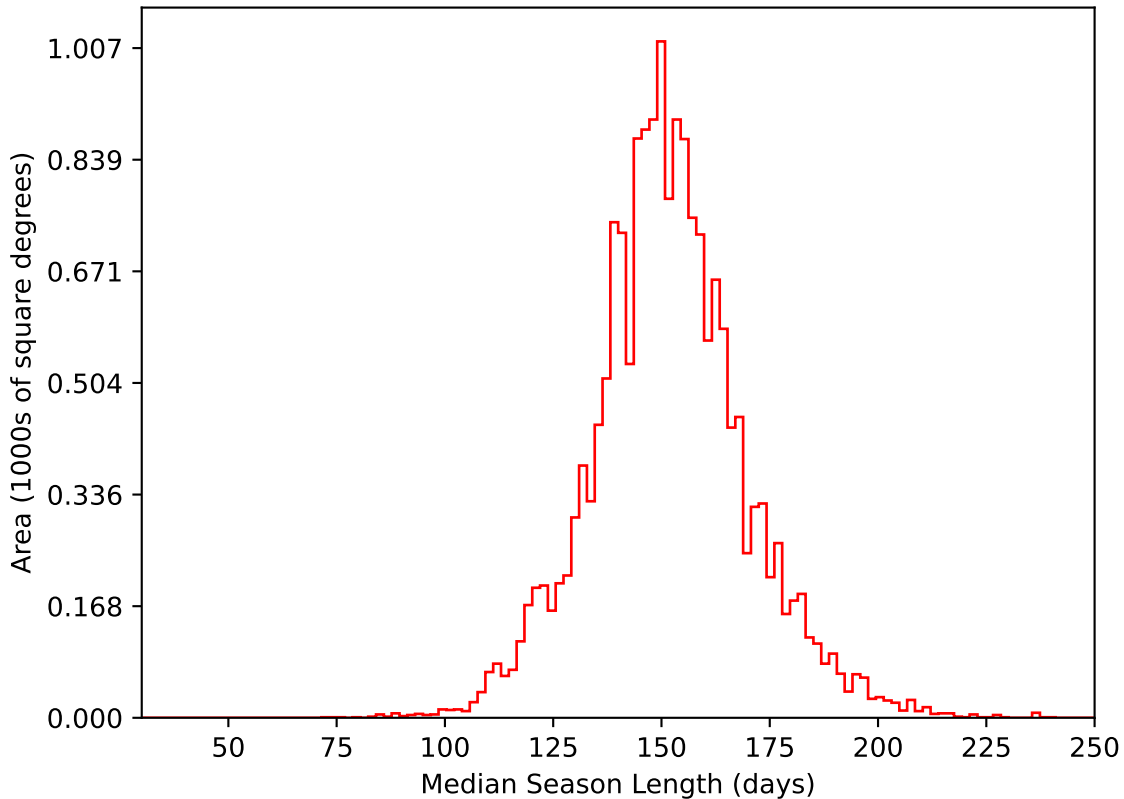
roll_pause_mjdp180_v3.4_10yrs WFD i band: Median Season Length
