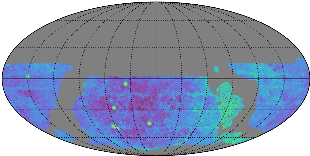
roll_pause_mjdp180_v3.4_10yrs WFD g band: Median Season Length
