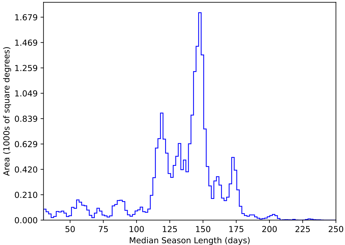
roll_pause_mjdp180_v3.4_10yrs All sky y band: Median Season Length
