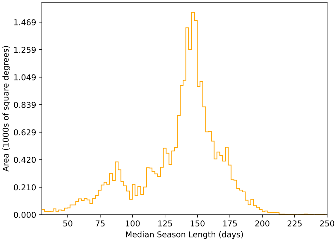
roll_pause_mjdp180_v3.4_10yrs All sky r band: Median Season Length
