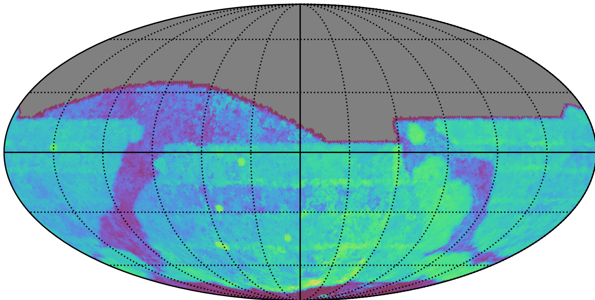
roll_pause_mjdp180_v3.4_10yrs All sky i band: Median Season Length
