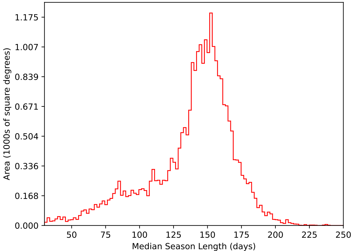
roll_pause_mjdp180_v3.4_10yrs All sky i band: Median Season Length
