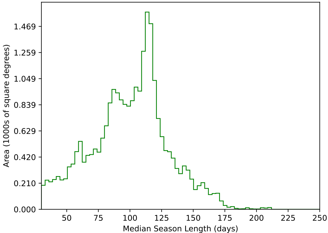
roll_pause_mjdp180_v3.4_10yrs All sky g band: Median Season Length
