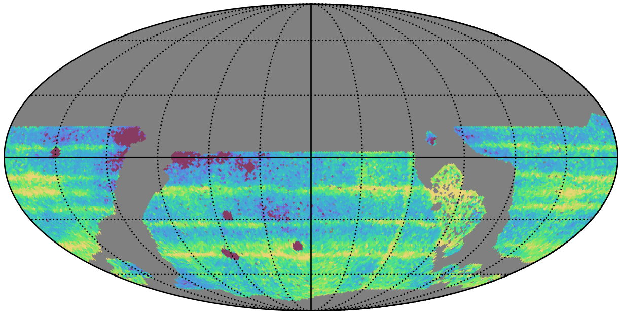
roll_pause_mjdp180_v3.4_10yrs WFD: Median Intra-Night Gap
