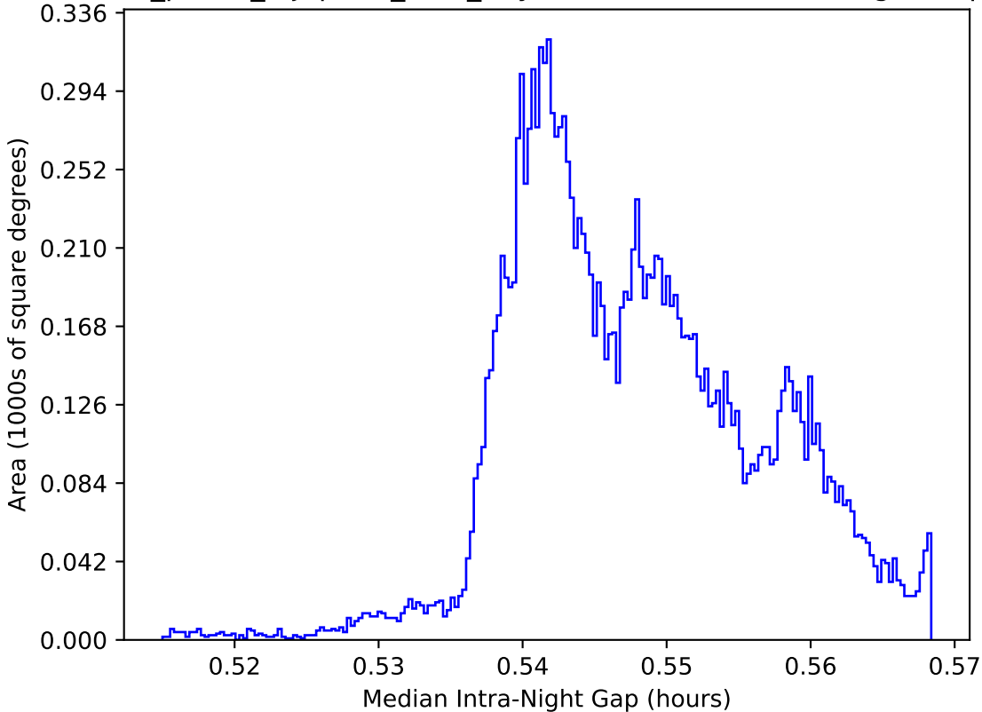
roll_pause_mjdp180_v3.4_10yrs WFD: Median Intra-Night Gap
