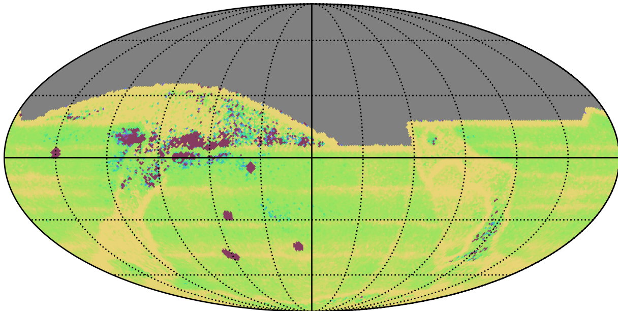
roll_pause_mjdp180_v3.4_10yrs All sky: Median Intra-Night Gap
