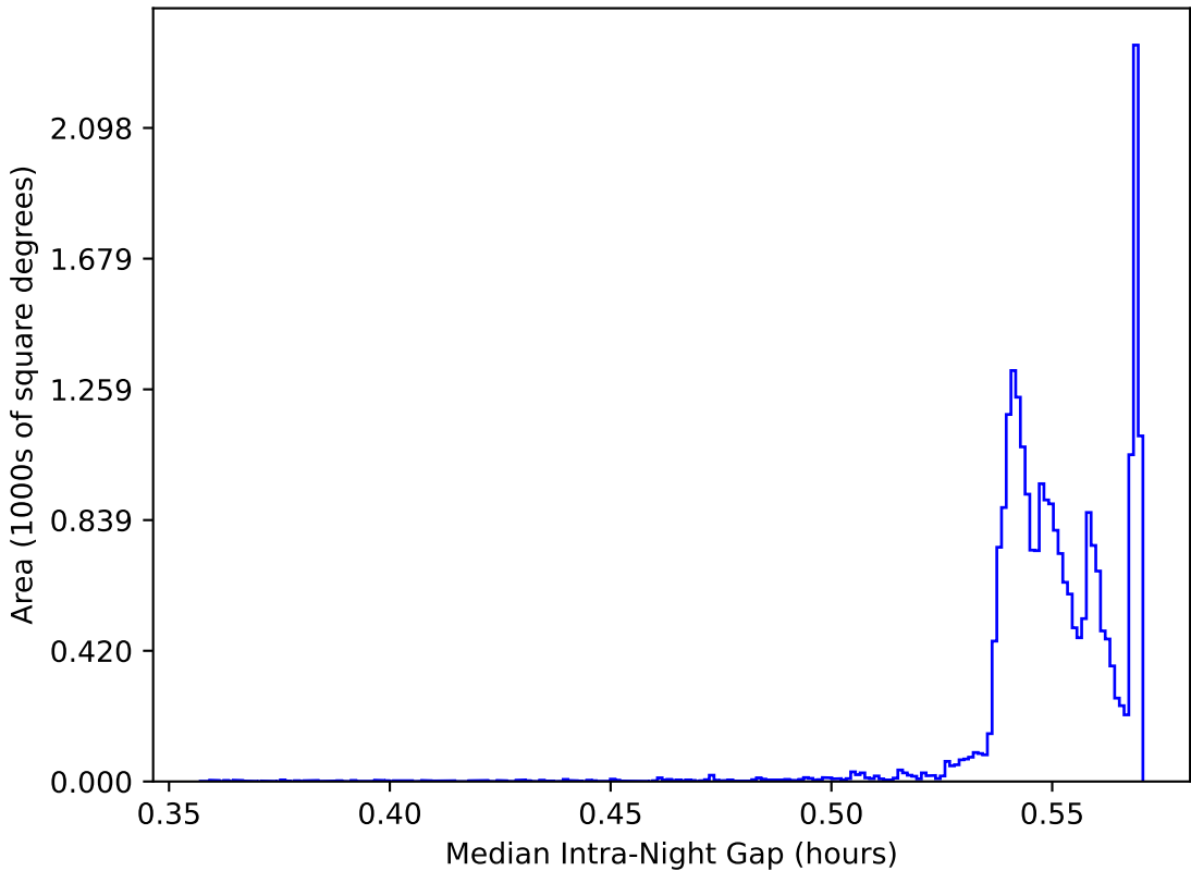
roll_pause_mjdp180_v3.4_10yrs All sky: Median Intra-Night Gap
