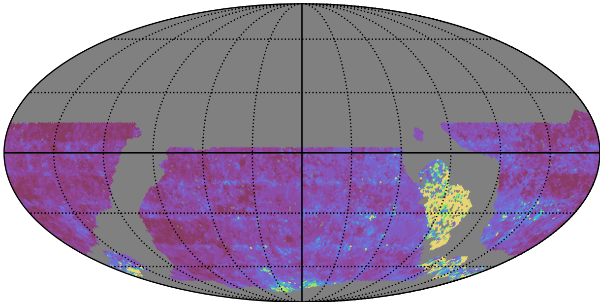
roll_pause_mjdp180_v3.4_10yrs WFD u band: Median Inter-Night Gap
