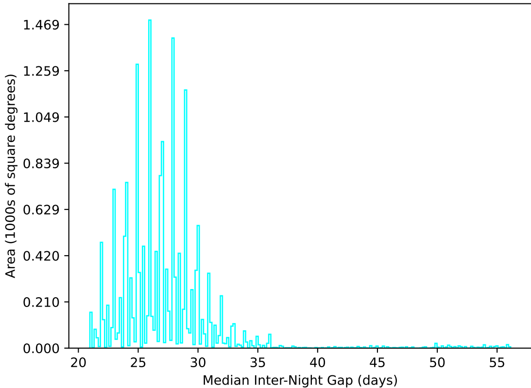
roll_pause_mjdp180_v3.4_10yrs WFD u band: Median Inter-Night Gap
