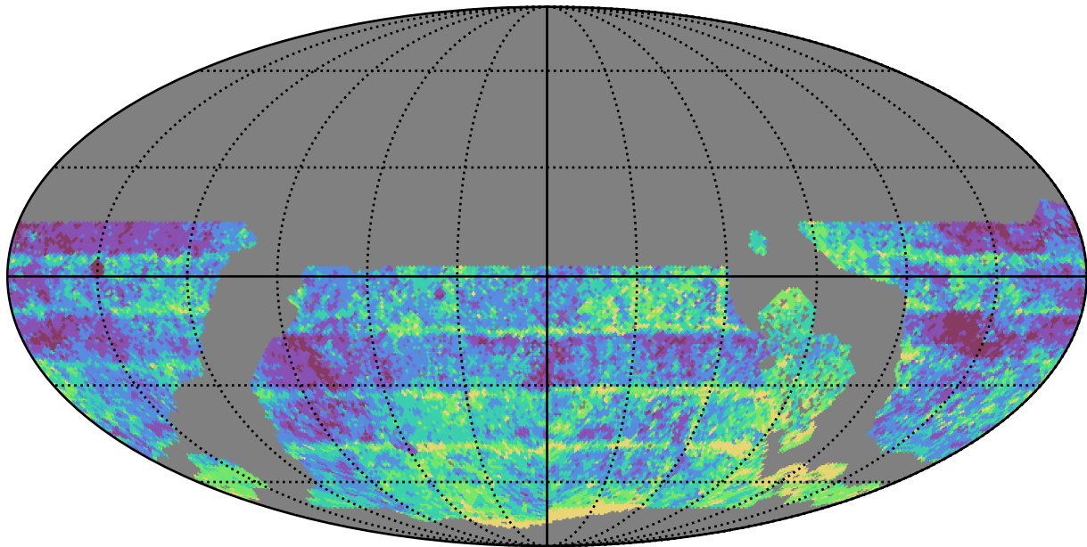
roll_pause_mjdp180_v3.4_10yrs WFD r band: Median Inter-Night Gap
