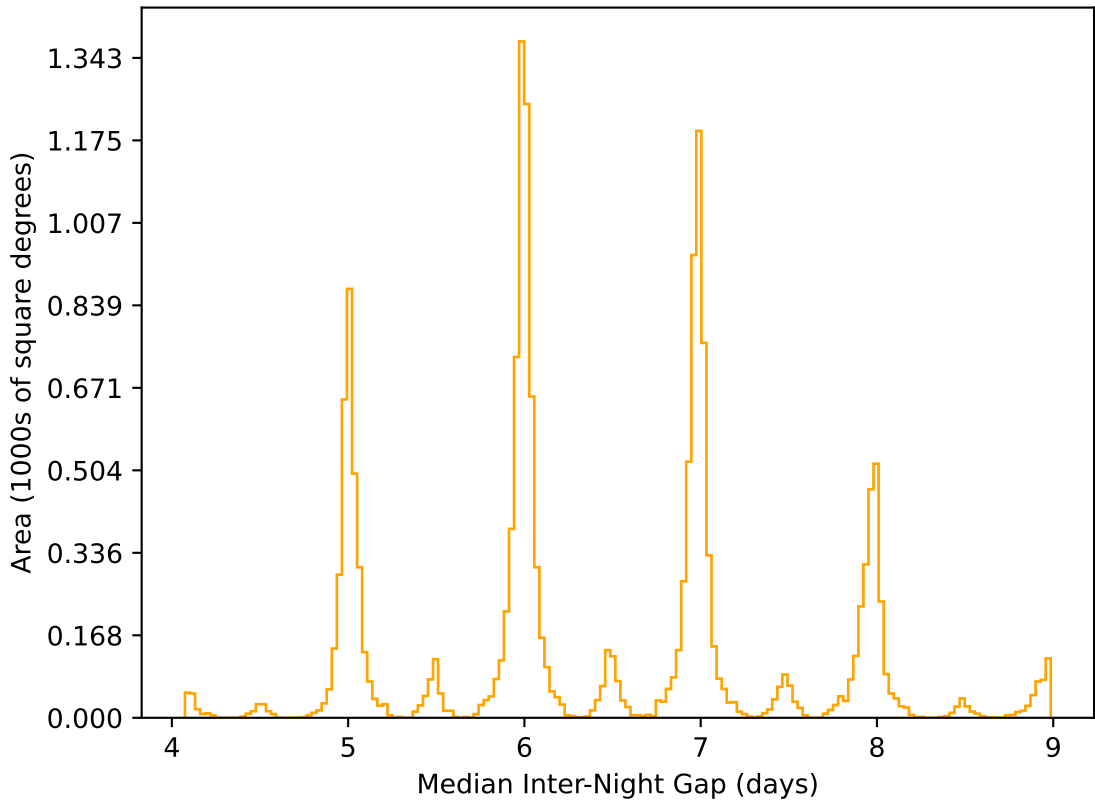
roll_pause_mjdp180_v3.4_10yrs WFD r band: Median Inter-Night Gap
