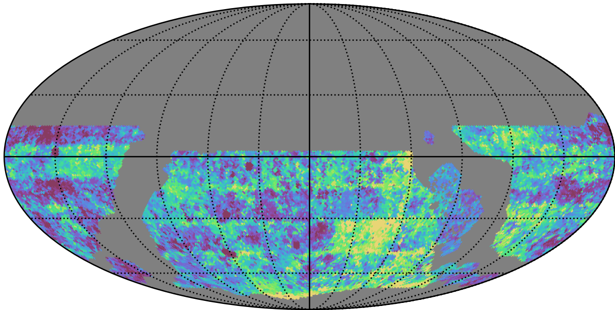
roll_pause_mjdp180_v3.4_10yrs WFD g band: Median Inter-Night Gap
