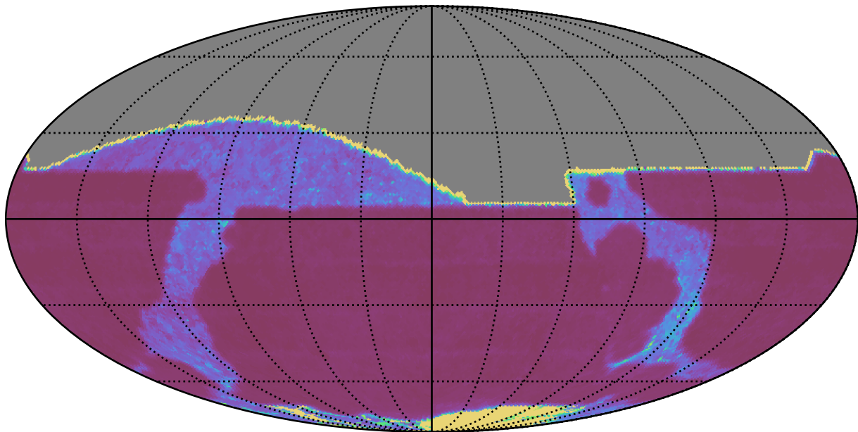
roll_pause_mjdp180_v3.4_10yrs All sky r band: Median Inter-Night Gap
